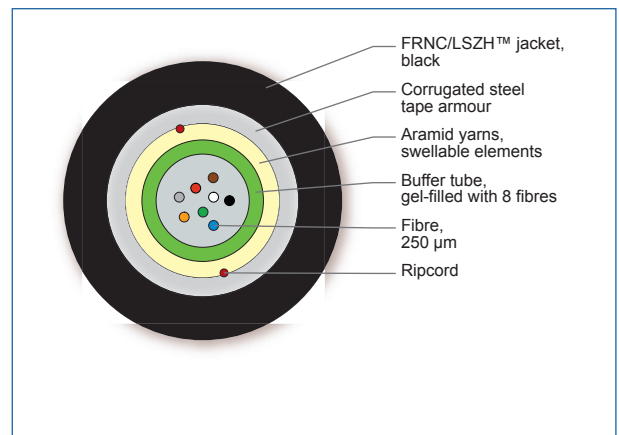
Cross Section of Order Number: 008TEY-13198A2G
