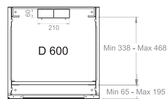
Max. / Min Equipment mounting distance (600)
