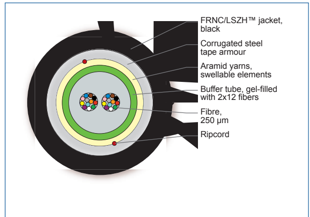
Cross Section of Order Number: 024TEY-13198A2G
